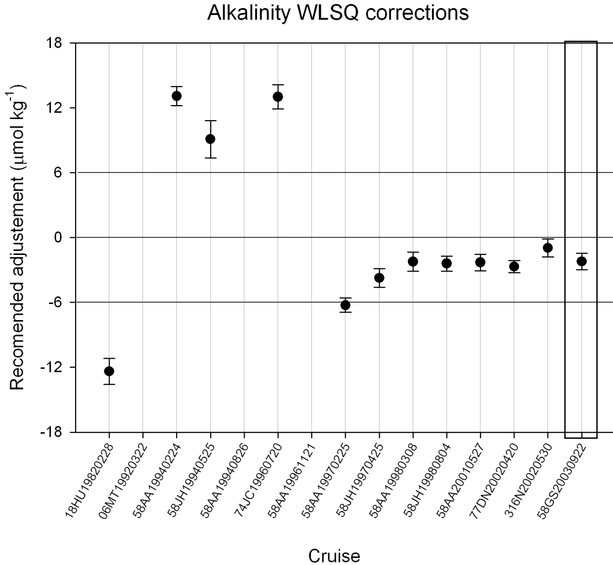
Figure 1: Recommended adjustments from WLSQ inversion of manual crossovers. Values are all in \mu\text{mol kg}^{-1} . Cut off for applying alkalinity correction is 6 \mu\text{mol kg}^{-1} as indicated with the lines in the figure.
